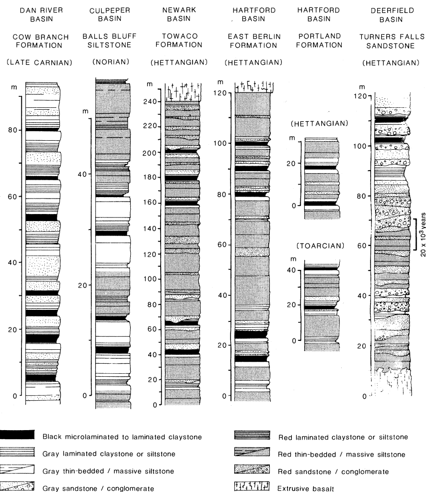
Fig. 5. Comparisons of sequences from various portions of the Newark Supergroup other than the Lockatong and Passaic formations (37, 38), all shown with the Van Houten cycles drawn to the same time scale. With the exception of the Portland Formation intervals, each section shows two 100,000-year cycles.
